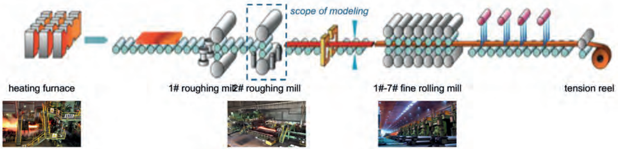
Figure 15: Hot milling process flow of Baosteel 1580 plant
